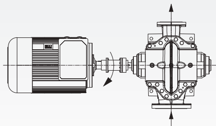
Direction of rotation clockwise (Motor from the drive end)
