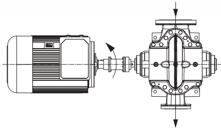
Direction of rotation counter clockwise (Motor from the drive end)
