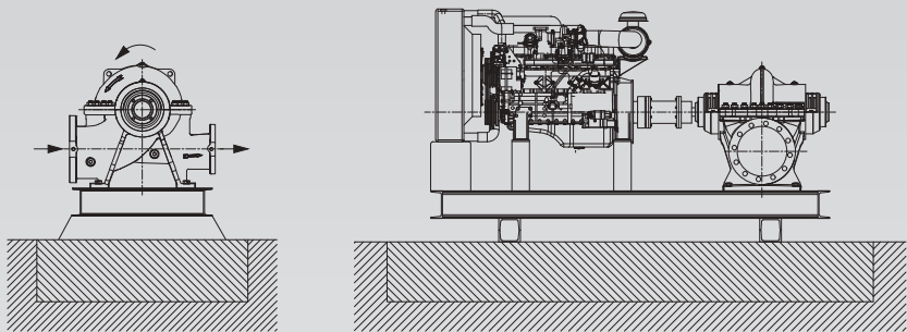
PUMP INSTALLATION WITH DIESEL
