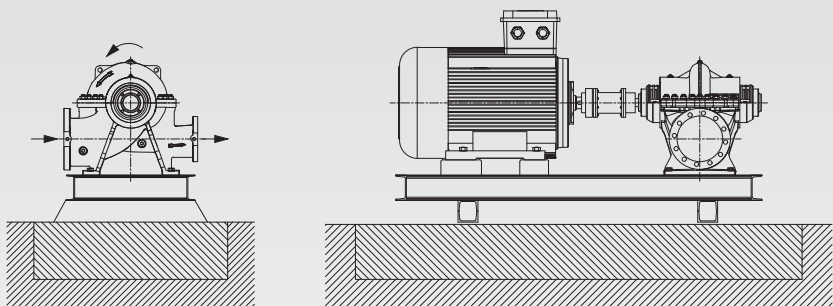
PUMP INSTALLATION WITH ELECTRIC MOTOR
