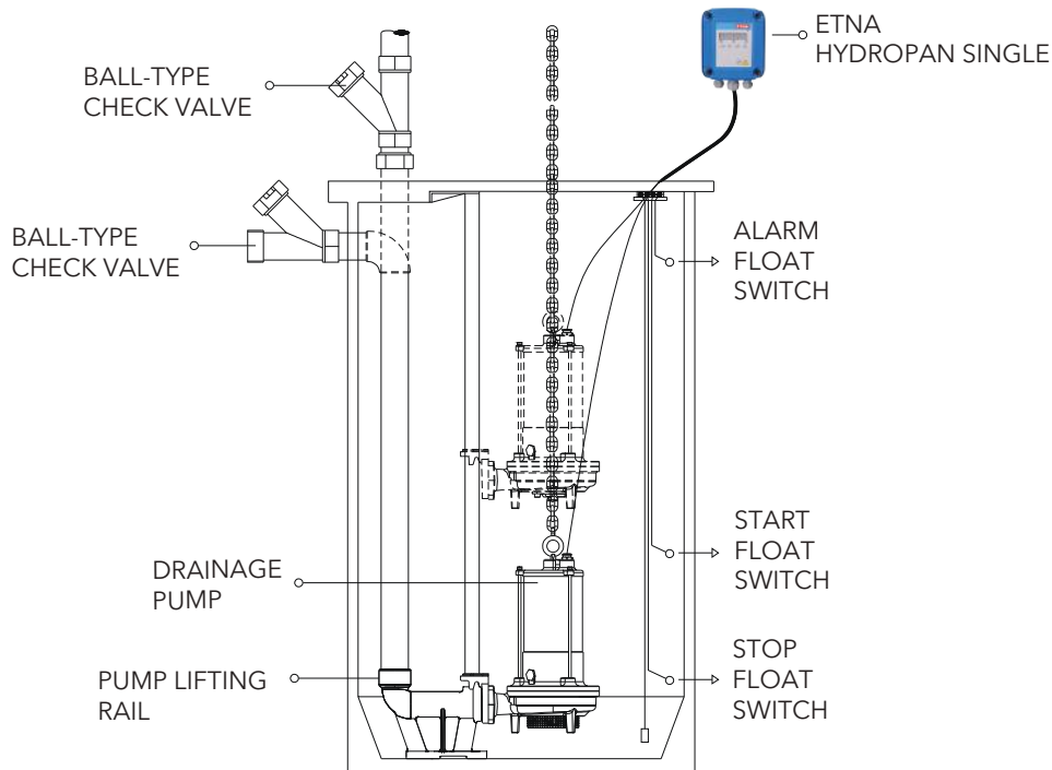
Fixed Installation with Lifting Rail (Pump can be removed for easy maintenance and repair)
